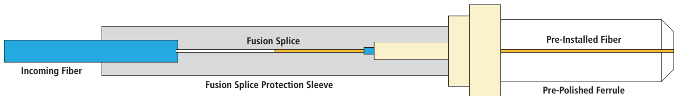
Figure 2—FUSEConnect SC, FC, LC and ST Connectors
