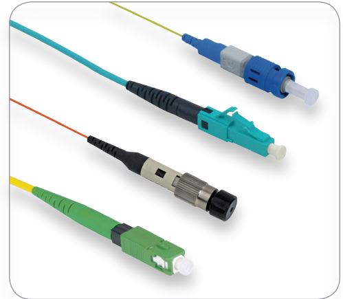
Figure 2—FUSEConnect SC, FC, LC and ST Connectors
